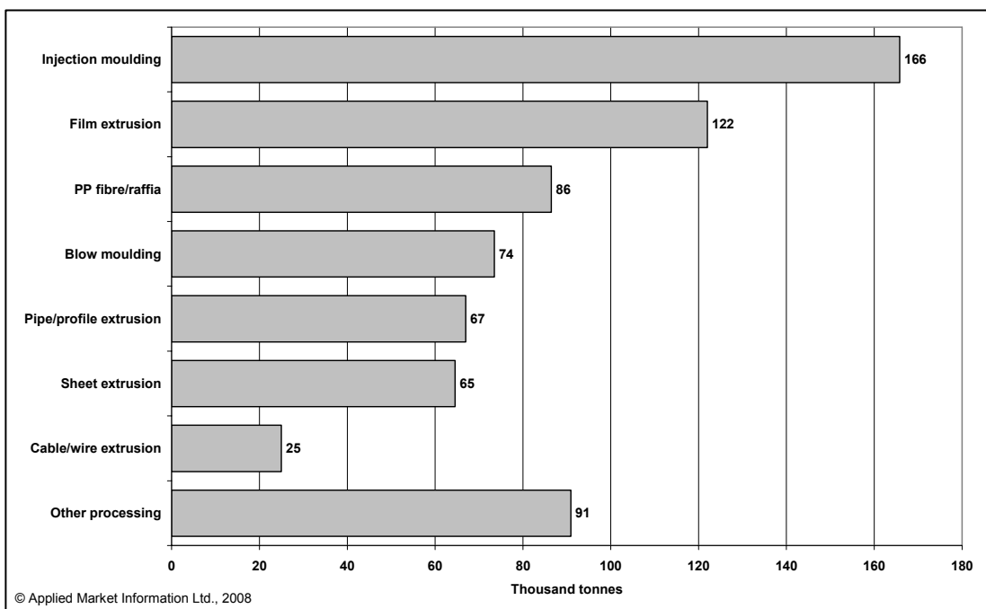
Figure 3: THERMOPLASTICS DEMAND IN CZECH REPUBLIC BY END USE PROCESS 2008
